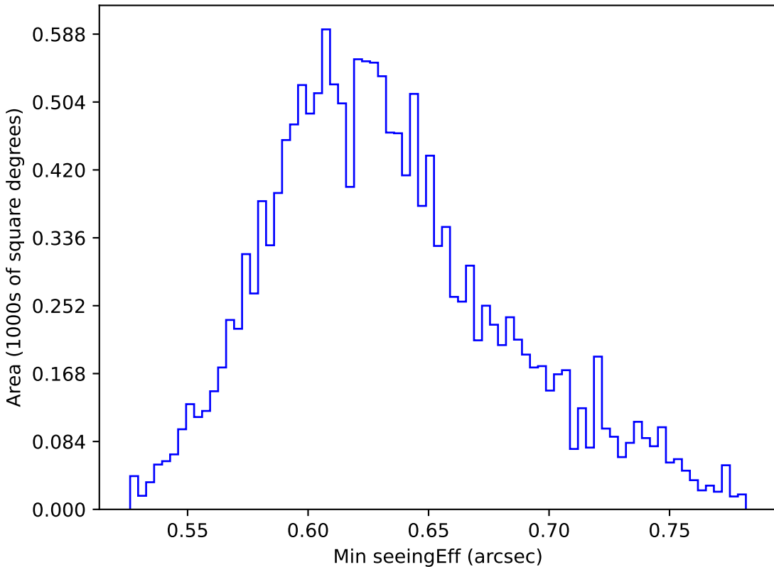
scp_reweight_v3.3_10yrs WFD y band: Min seeingEff
