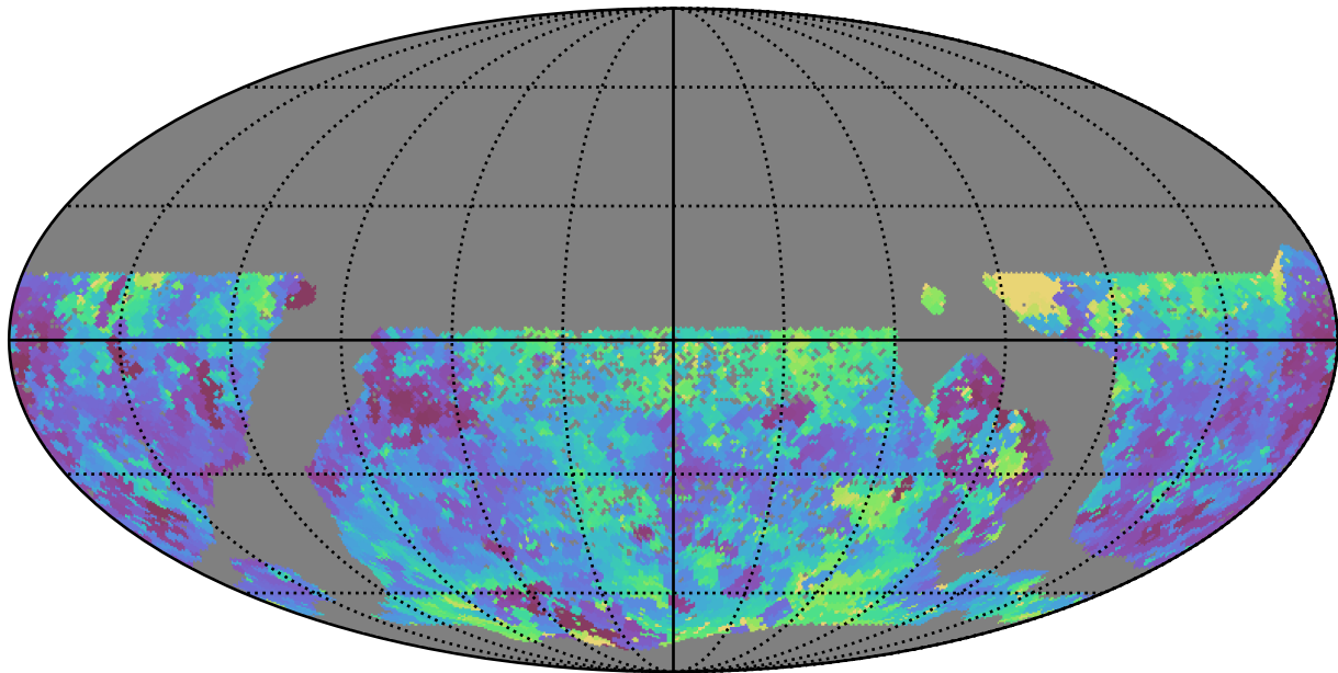
scp_reweight_v3.3_10yrs WFD u band: Min seeingEff
