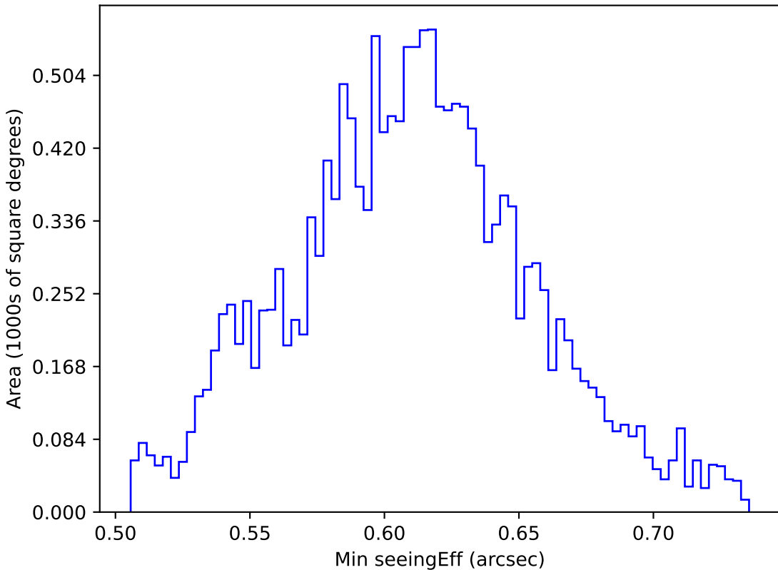
scp_reweight_v3.3_10yrs WFD r band: Min seeingEff
