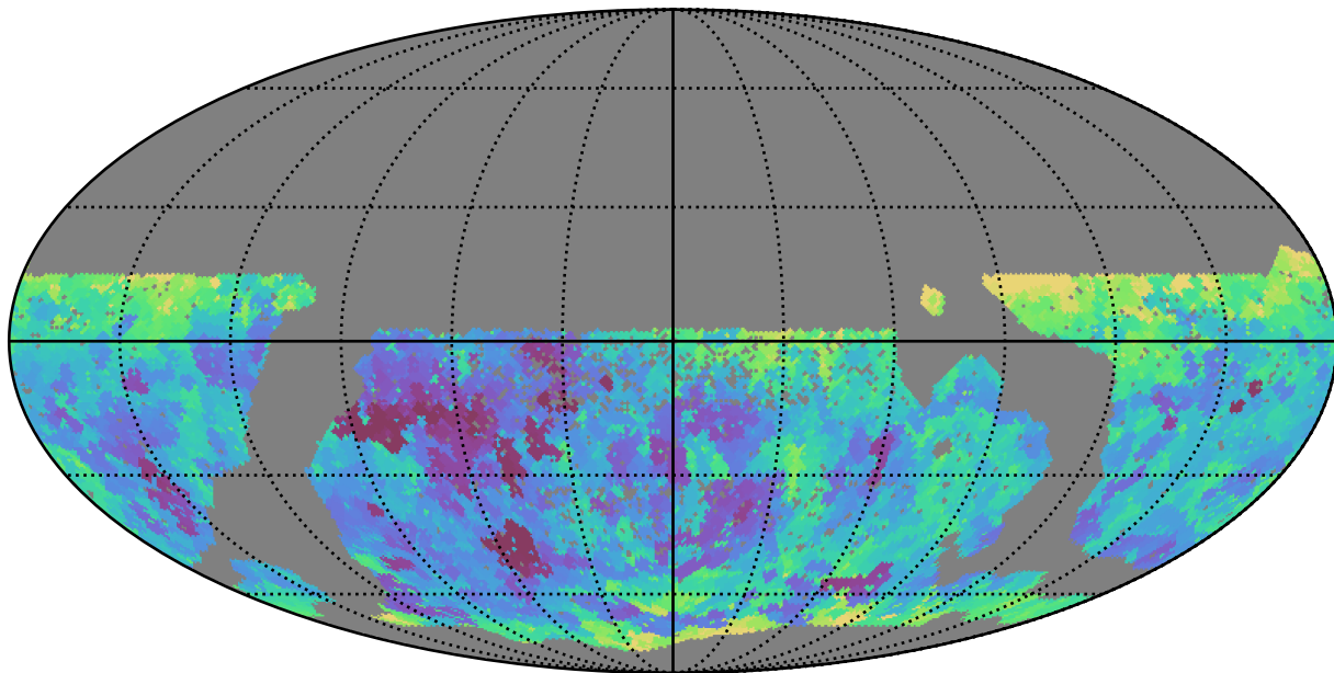
scp_reweight_v3.3_10yrs WFD i band: Min seeingEff
