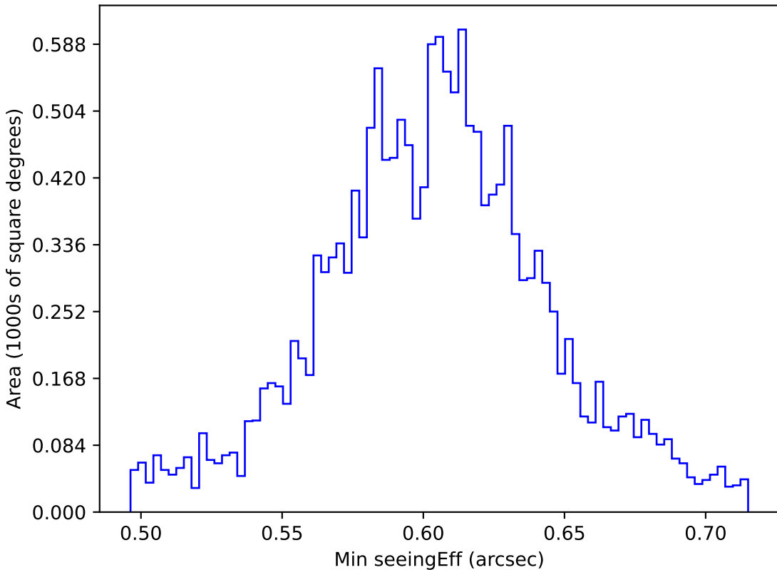
scp_reweight_v3.3_10yrs WFD i band: Min seeingEff
