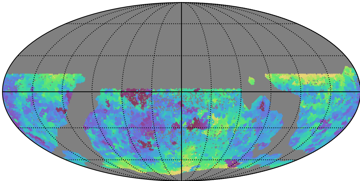
scp_reweight_v3.3_10yrs WFD g band: Min seeingEff
