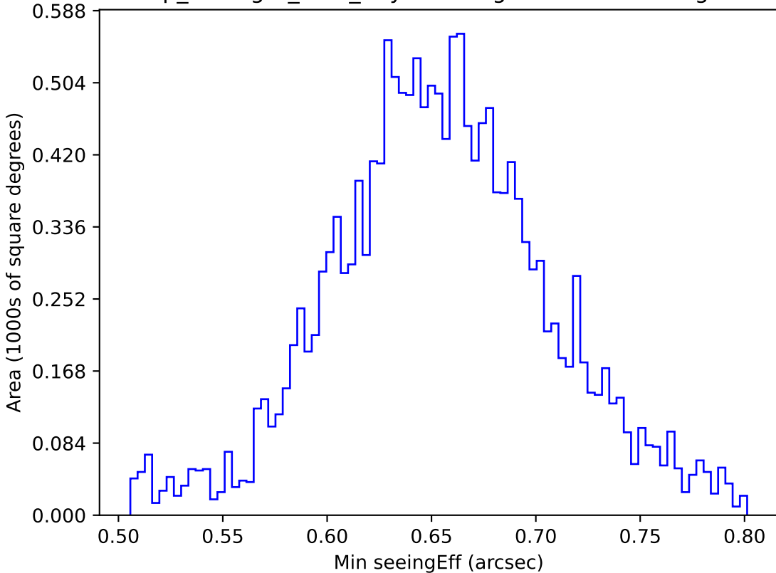
scp_reweight_v3.3_10yrs WFD g band: Min seeingEff
