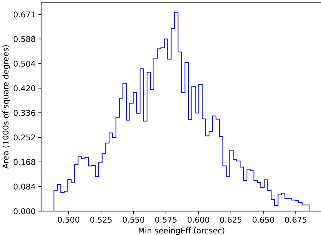
scp_reweight_v3.3_10yrs WFD all bands: Min seeingEff
