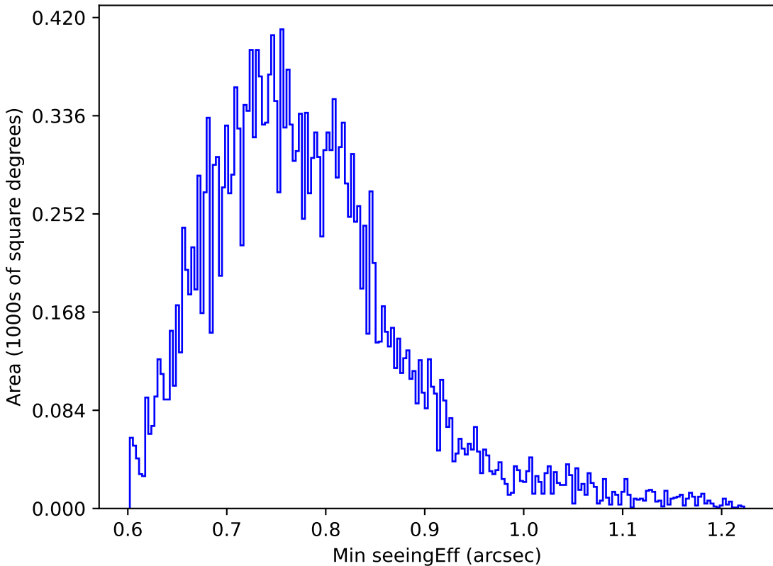
scp_reweight_v3.3_10yrs All sky u band: Min seeingEff
