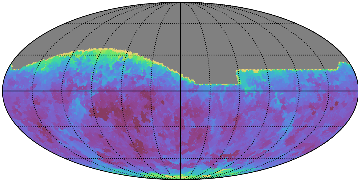
scp_reweight_v3.3_10yrs All sky i band: Min seeingEff
