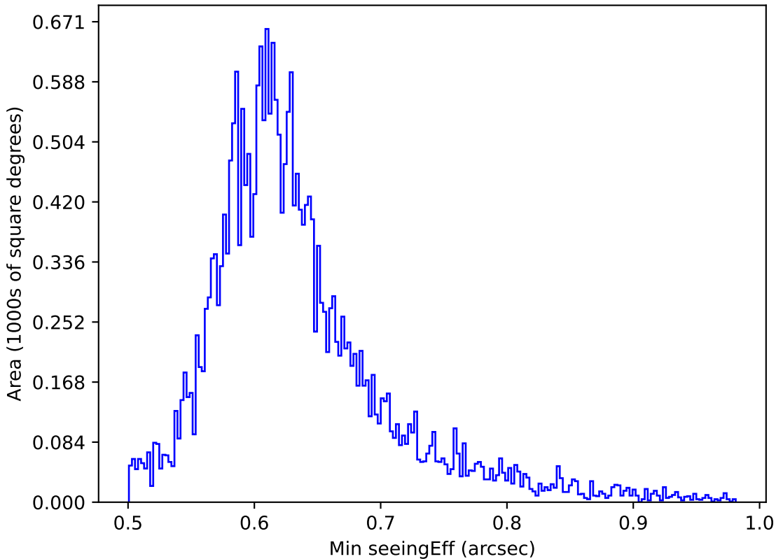
scp_reweight_v3.3_10yrs All sky i band: Min seeingEff
