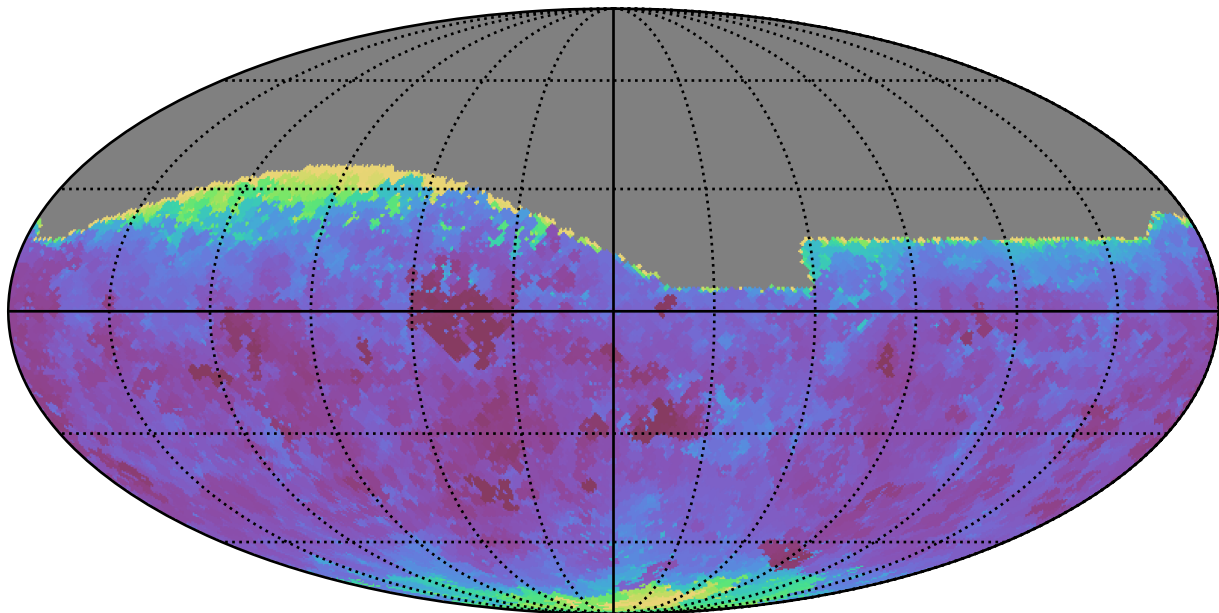
scp_reweight_v3.3_10yrs All sky g band: Min seeingEff
