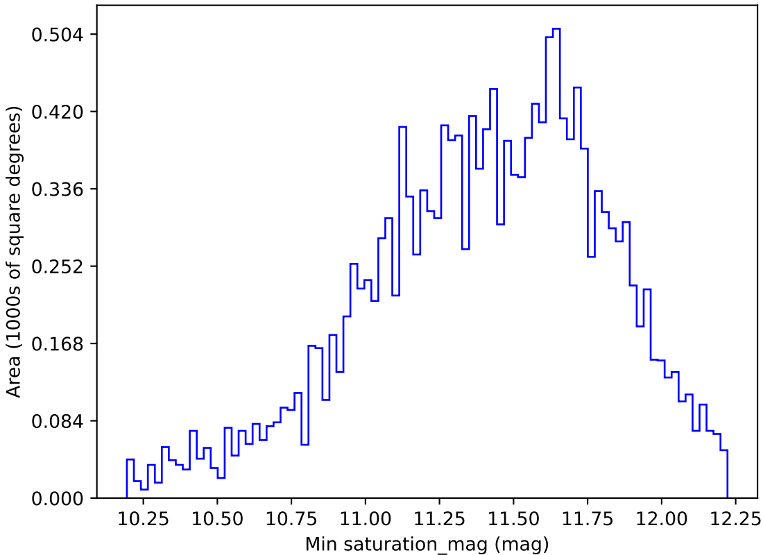
scp_reweight_v3.3_10yrs WFD u band: Min saturation_mag
