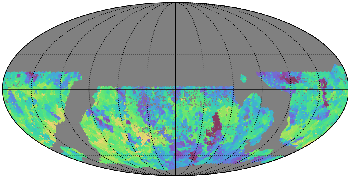
scp_reweight_v3.3_10yrs WFD i band: Min saturation_mag
