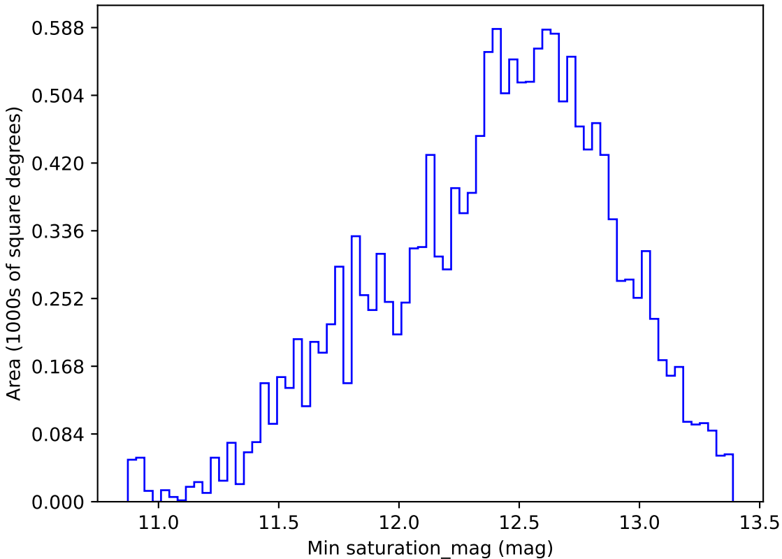
scp_reweight_v3.3_10yrs WFD i band: Min saturation_mag
