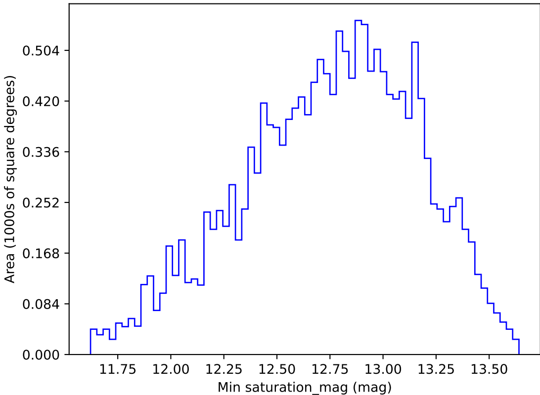
scp_reweight_v3.3_10yrs WFD g band: Min saturation_mag
