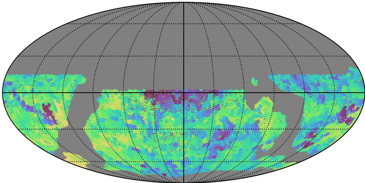
scp_reweight_v3.3_10yrs WFD all bands: Min saturation_mag
