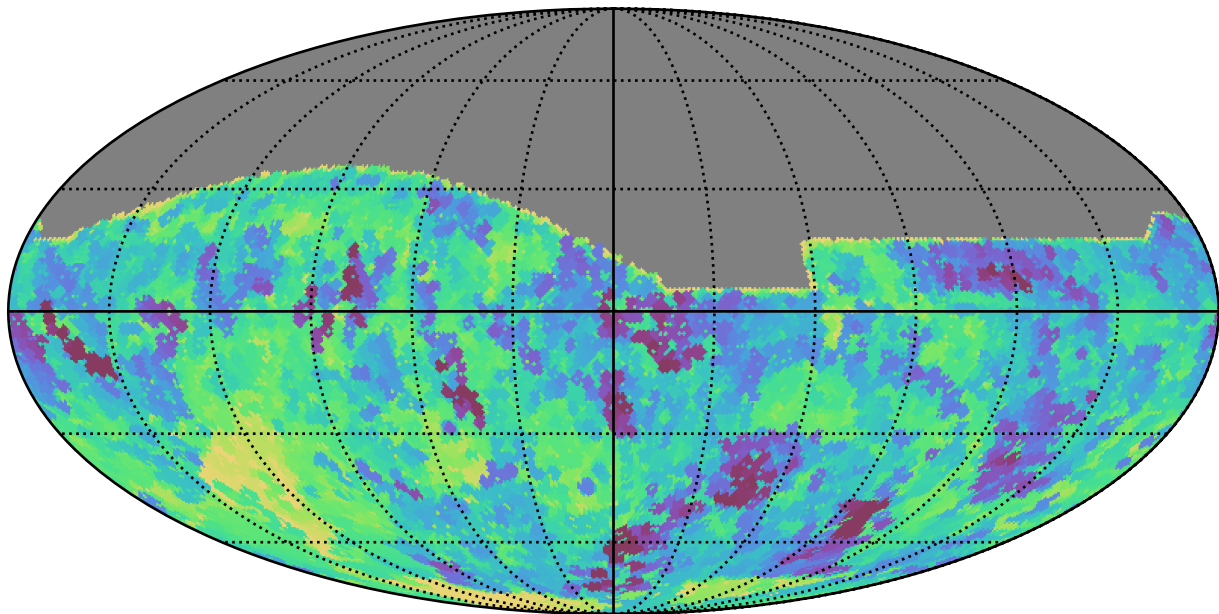
scp_reweight_v3.3_10yrs All sky z band: Min saturation_mag
