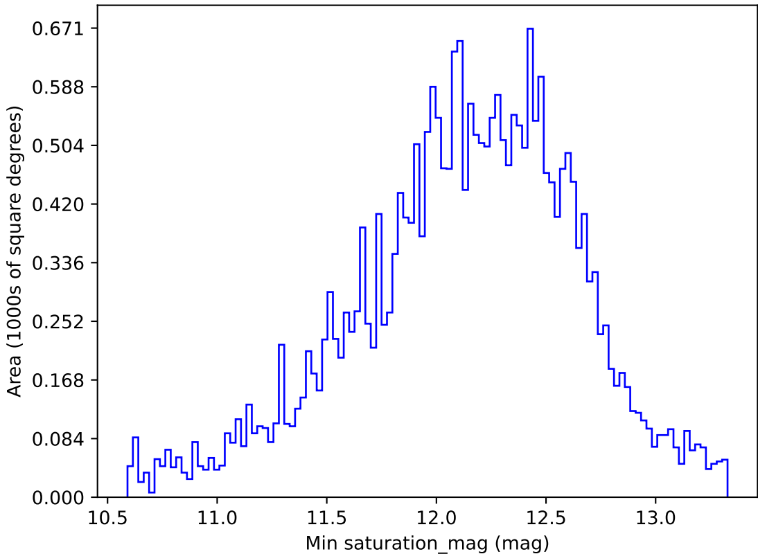
scp_reweight_v3.3_10yrs All sky z band: Min saturation_mag
