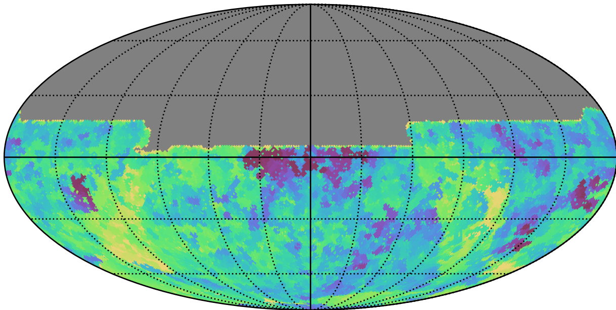
scp_reweight_v3.3_10yrs All sky y band: Min saturation_mag
