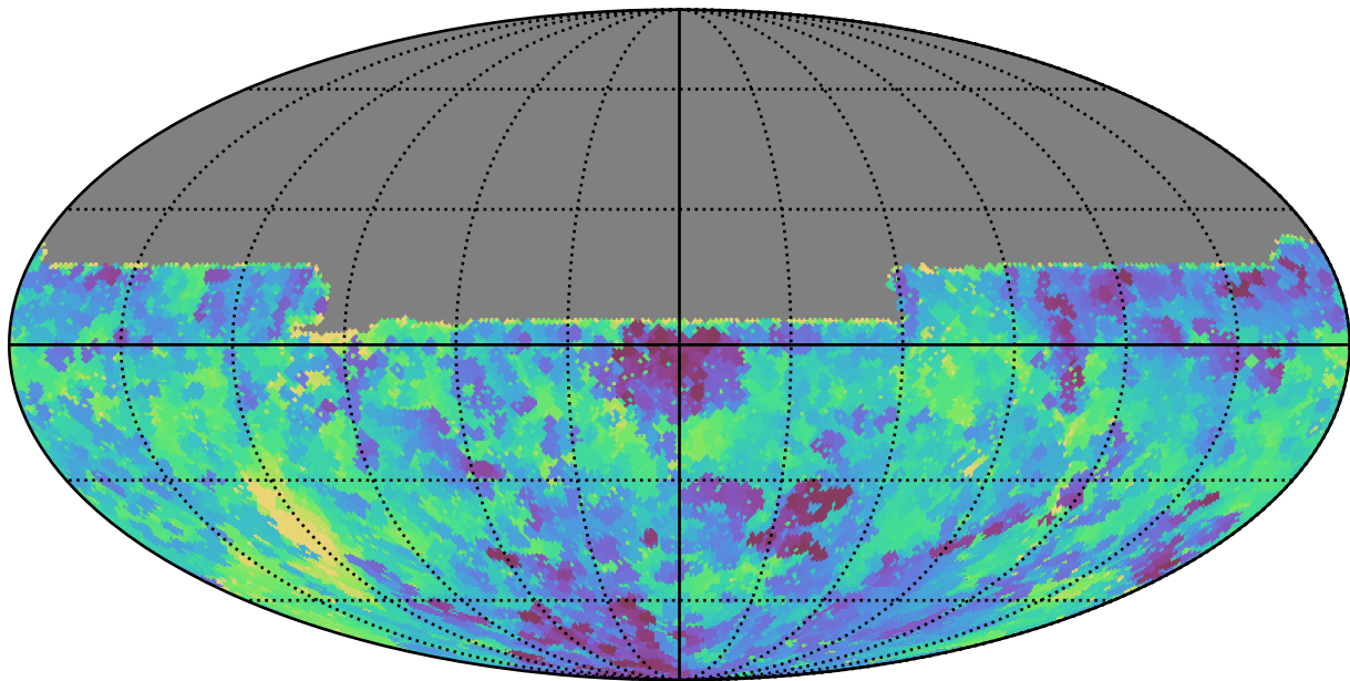
scp_reweight_v3.3_10yrs All sky u band: Min saturation_mag
