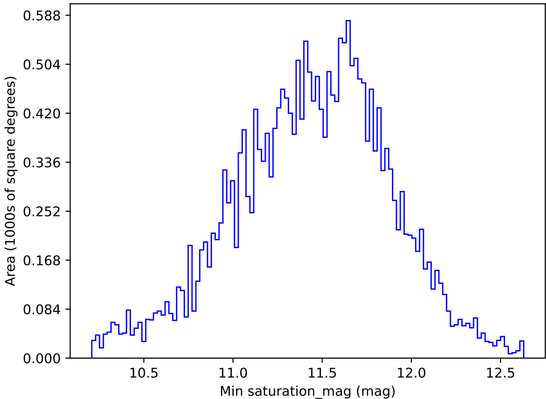
scp_reweight_v3.3_10yrs All sky u band: Min saturation_mag
