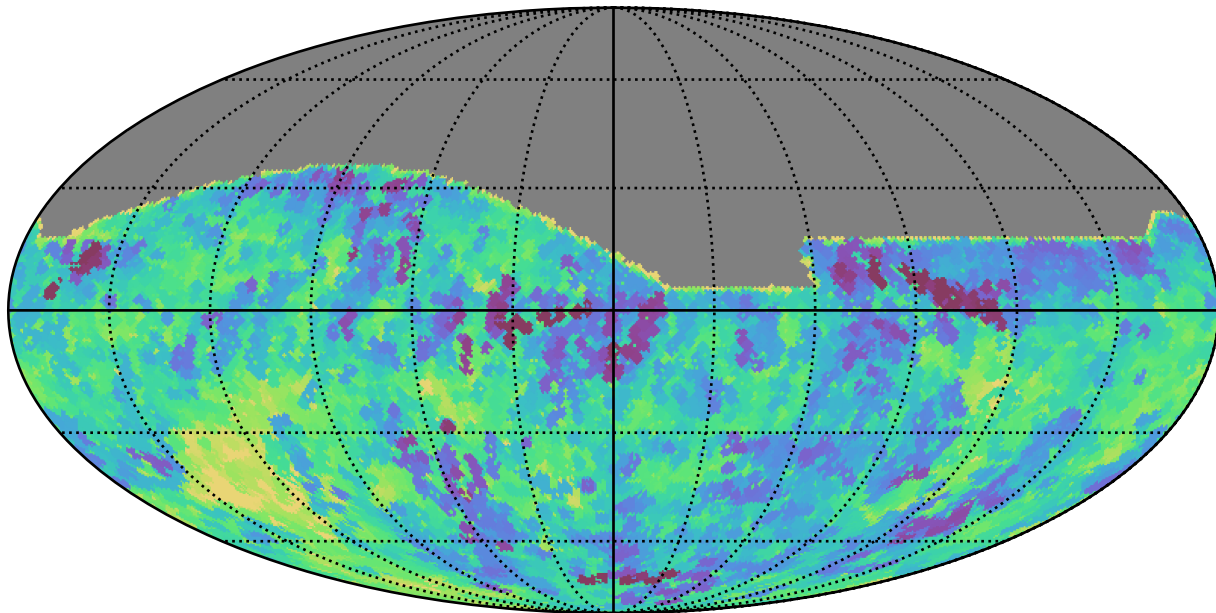
scp_reweight_v3.3_10yrs All sky r band: Min saturation_mag
