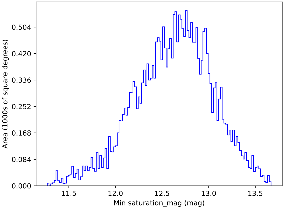
scp_reweight_v3.3_10yrs All sky r band: Min saturation_mag
