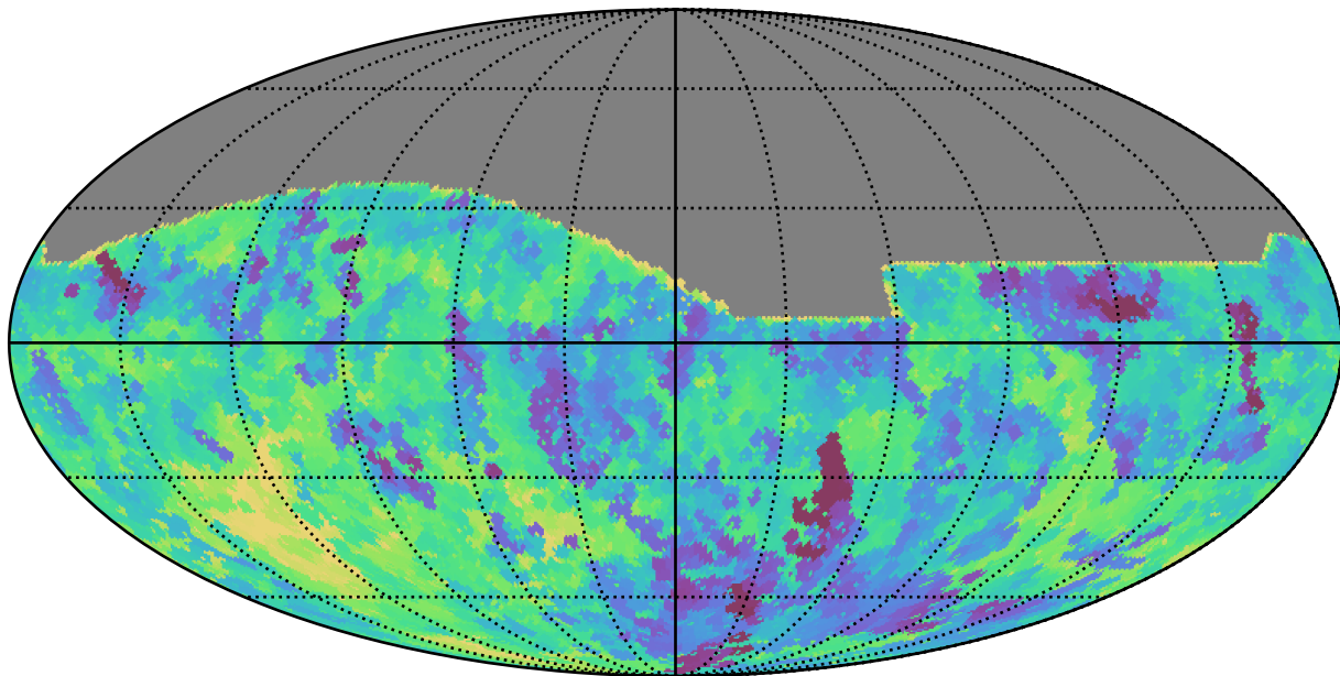
scp_reweight_v3.3_10yrs All sky i band: Min saturation_mag
