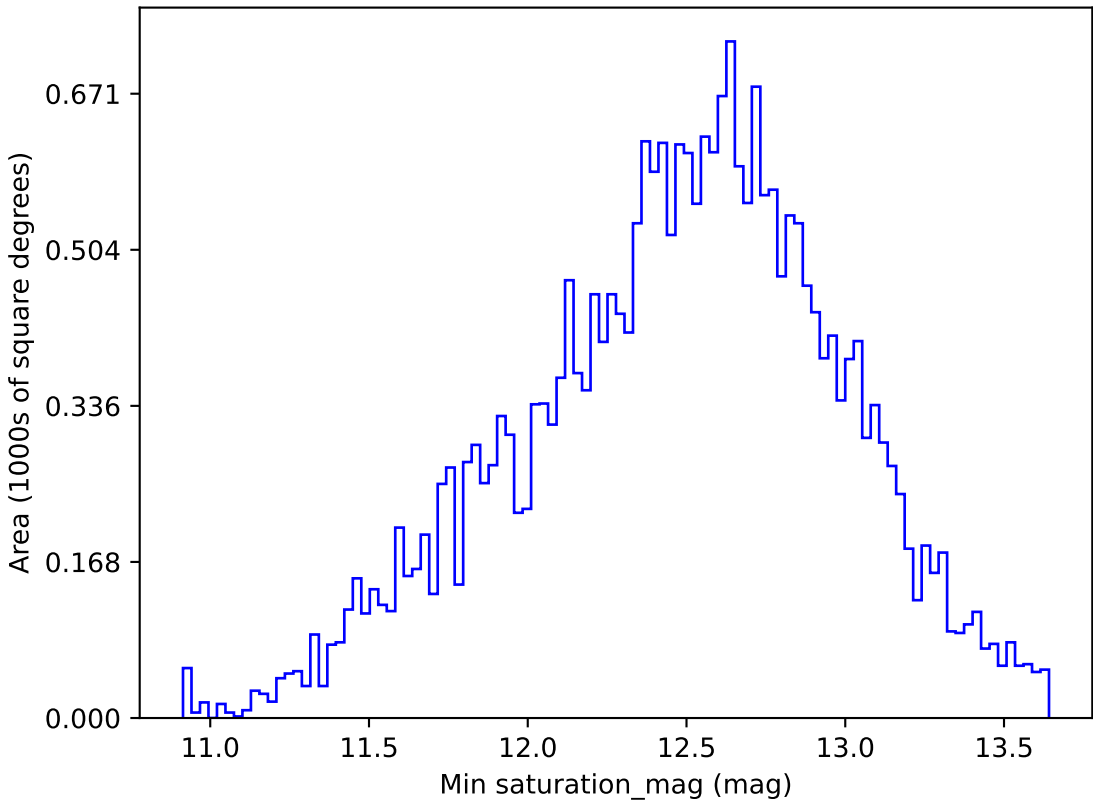
scp_reweight_v3.3_10yrs All sky i band: Min saturation_mag
