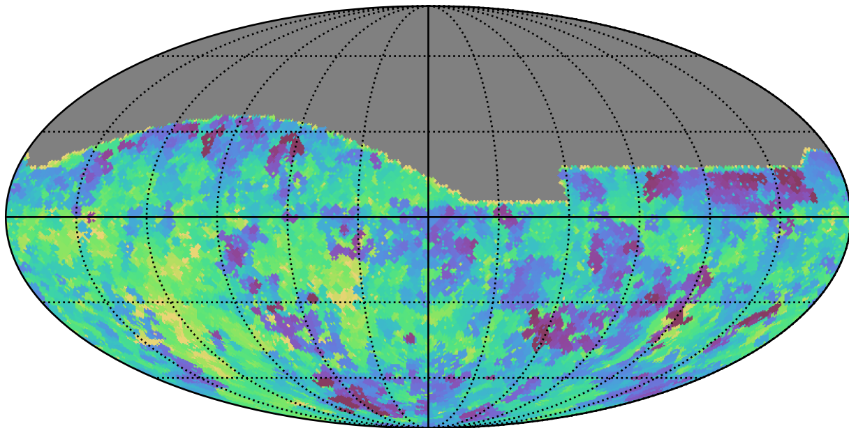
scp_reweight_v3.3_10yrs All sky g band: Min saturation_mag
