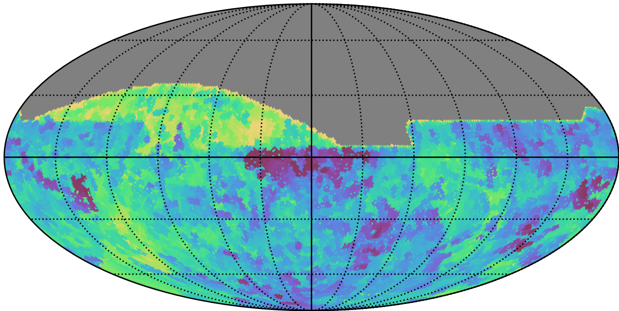
scp_reweight_v3.3_10yrs All sky all bands: Min saturation_mag
