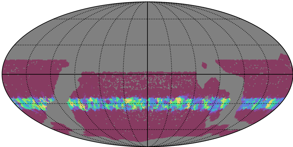
scp_reweight_v3.3_10yrs WFD z band: Min normairmass
