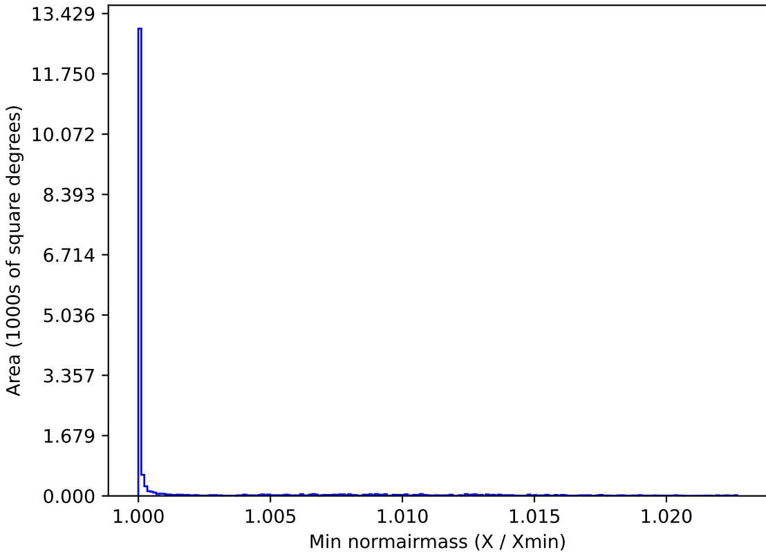
scp_reweight_v3.3_10yrs WFD z band: Min normairmass
