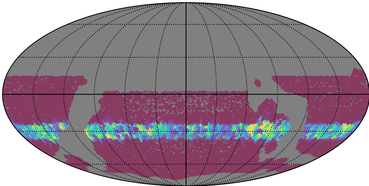
scp_reweight_v3.3_10yrs WFD y band: Min normairmass
