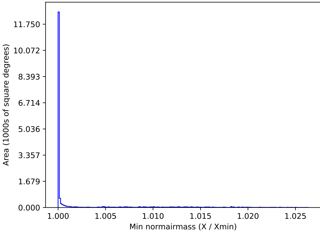
scp_reweight_v3.3_10yrs WFD y band: Min normairmass
