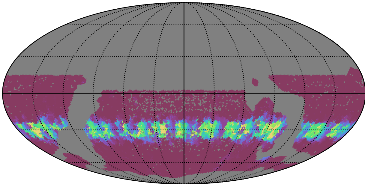
scp_reweight_v3.3_10yrs WFD u band: Min normairmass
