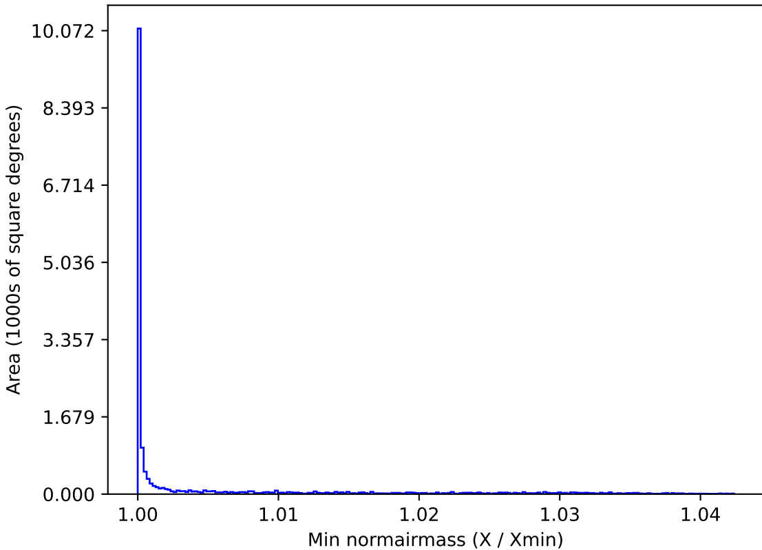
scp_reweight_v3.3_10yrs WFD u band: Min normairmass
