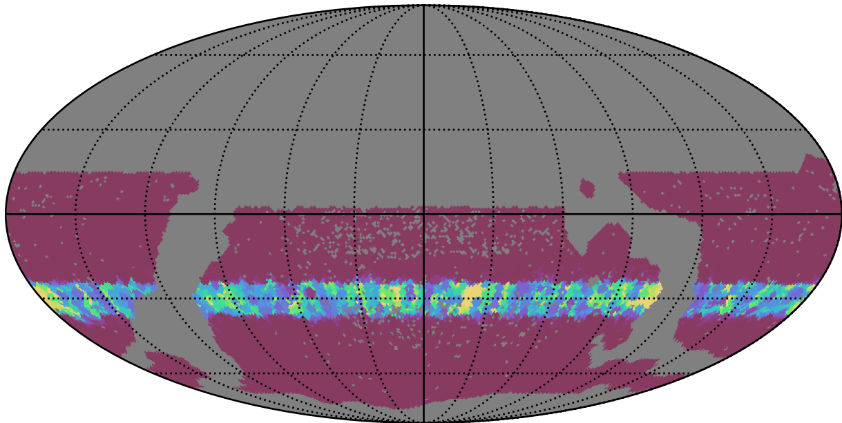
scp_reweight_v3.3_10yrs WFD i band: Min normairmass
