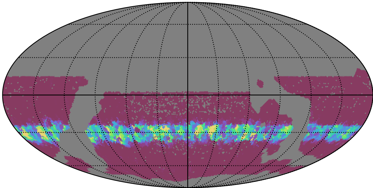
scp_reweight_v3.3_10yrs WFD g band: Min normairmass
