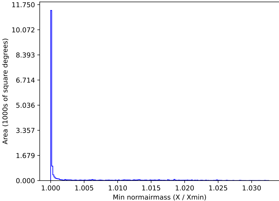
scp_reweight_v3.3_10yrs WFD g band: Min normairmass
