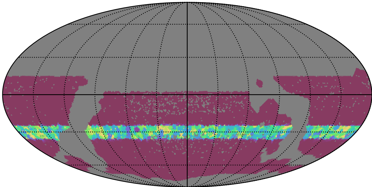
scp_reweight_v3.3_10yrs WFD all bands: Min normairmass
