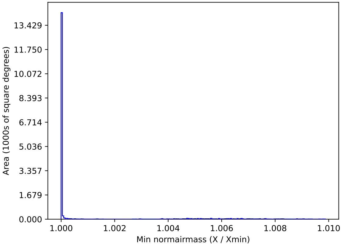
scp_reweight_v3.3_10yrs WFD all bands: Min normairmass
