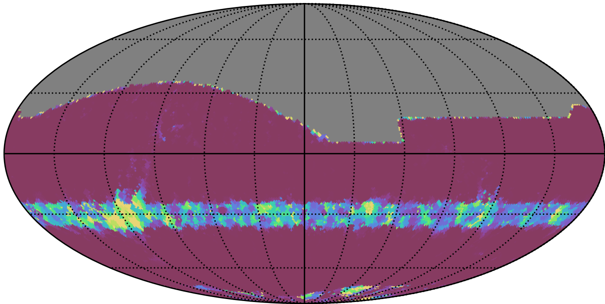
scp_reweight_v3.3_10yrs All sky z band: Min normairmass
