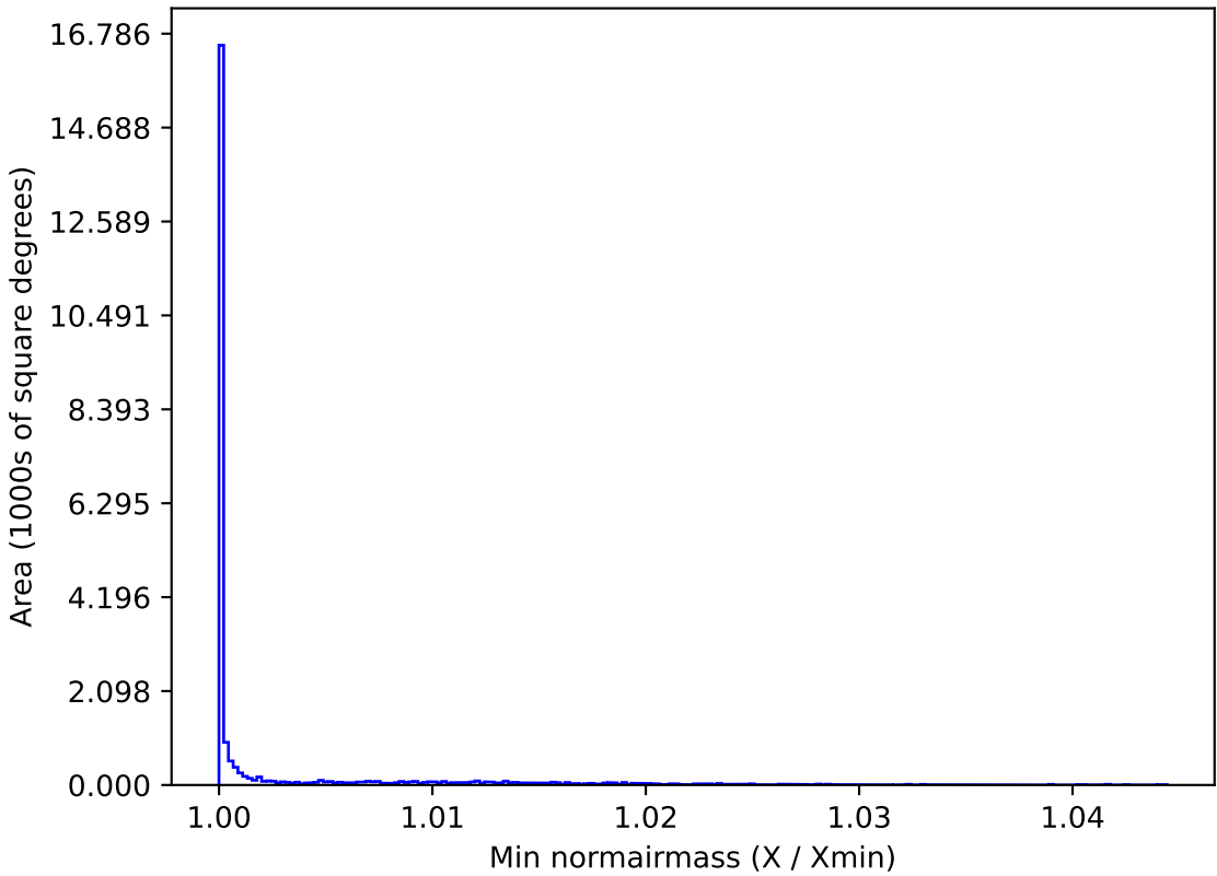
scp_reweight_v3.3_10yrs All sky y band: Min normairmass
