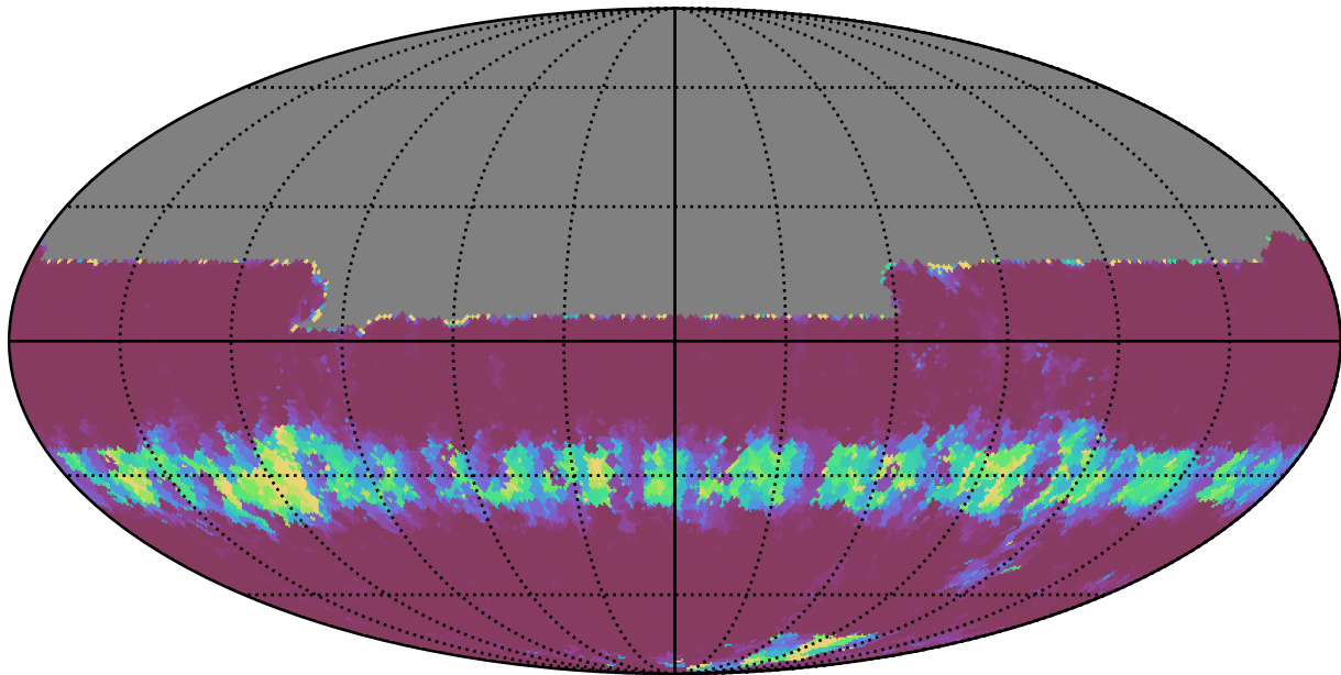
scp_reweight_v3.3_10yrs All sky u band: Min normairmass
