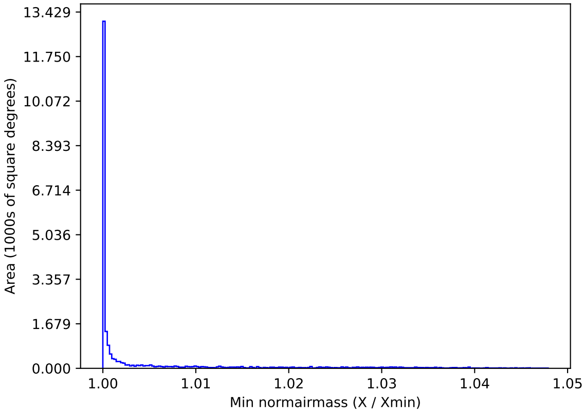
scp_reweight_v3.3_10yrs All sky u band: Min normairmass
