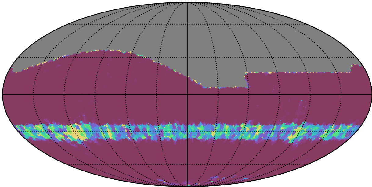
scp_reweight_v3.3_10yrs All sky r band: Min normairmass
