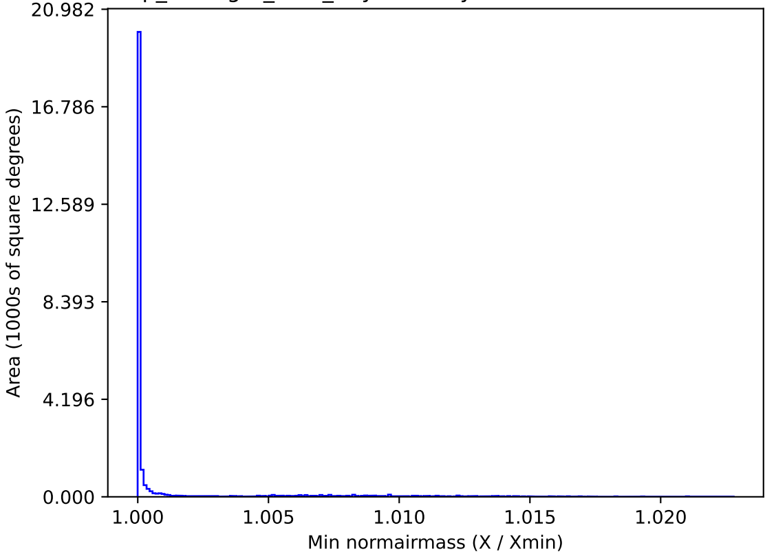
scp_reweight_v3.3_10yrs All sky i band: Min normairmass
