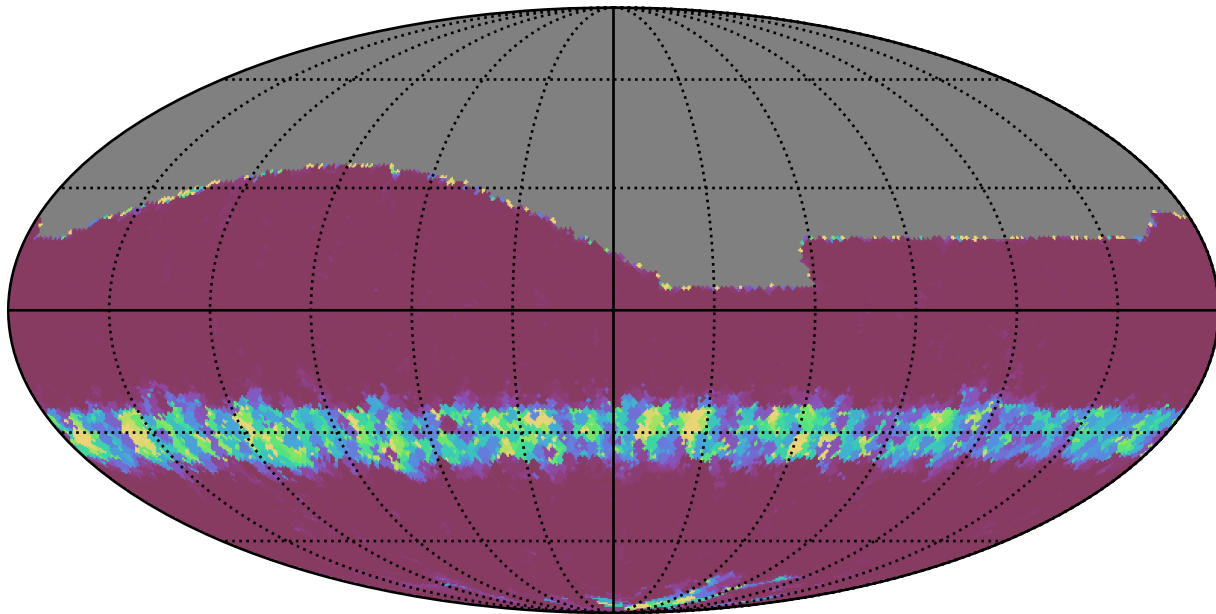
scp_reweight_v3.3_10yrs All sky g band: Min normairmass
