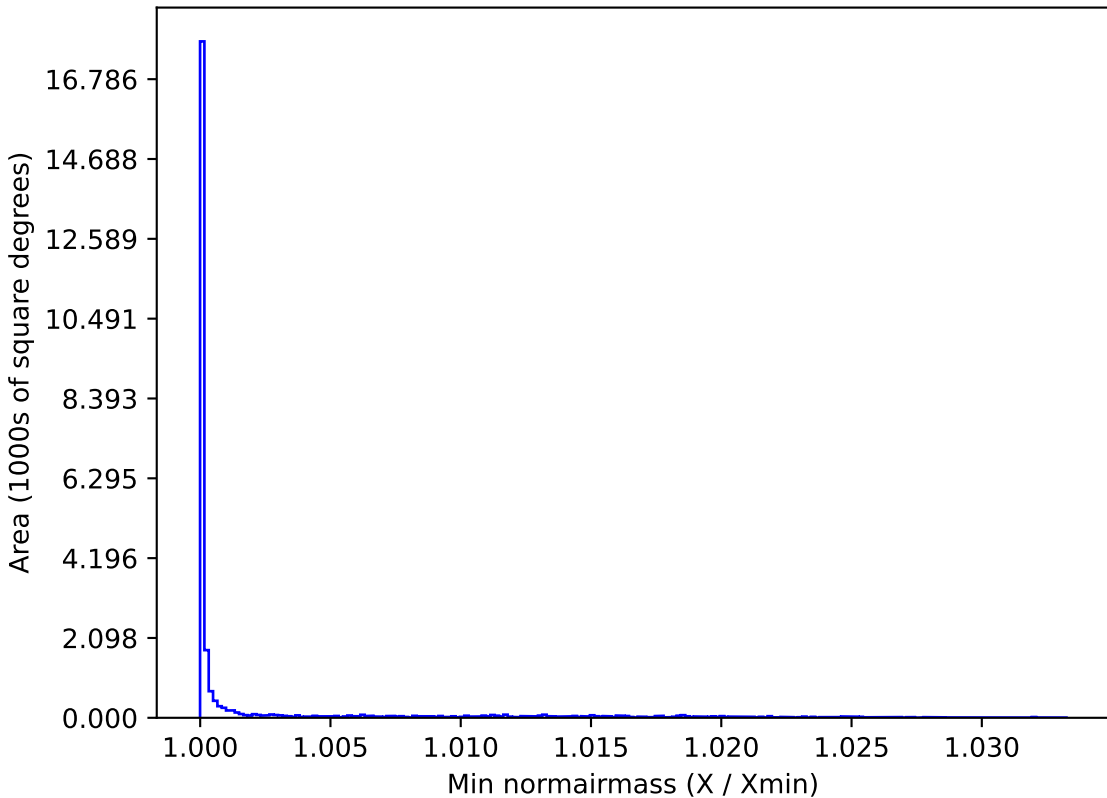
scp_reweight_v3.3_10yrs All sky g band: Min normairmass
