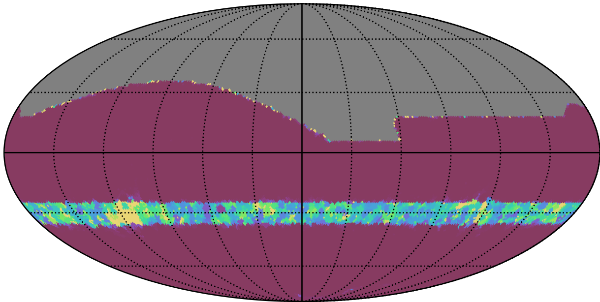
scp_reweight_v3.3_10yrs All sky all bands: Min normairmass
