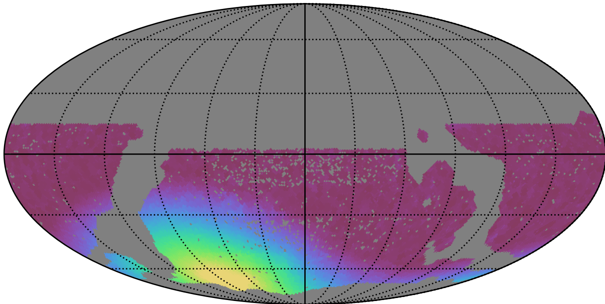
scp_reweight_v3.3_10yrs WFD z band: Min moonDistance
