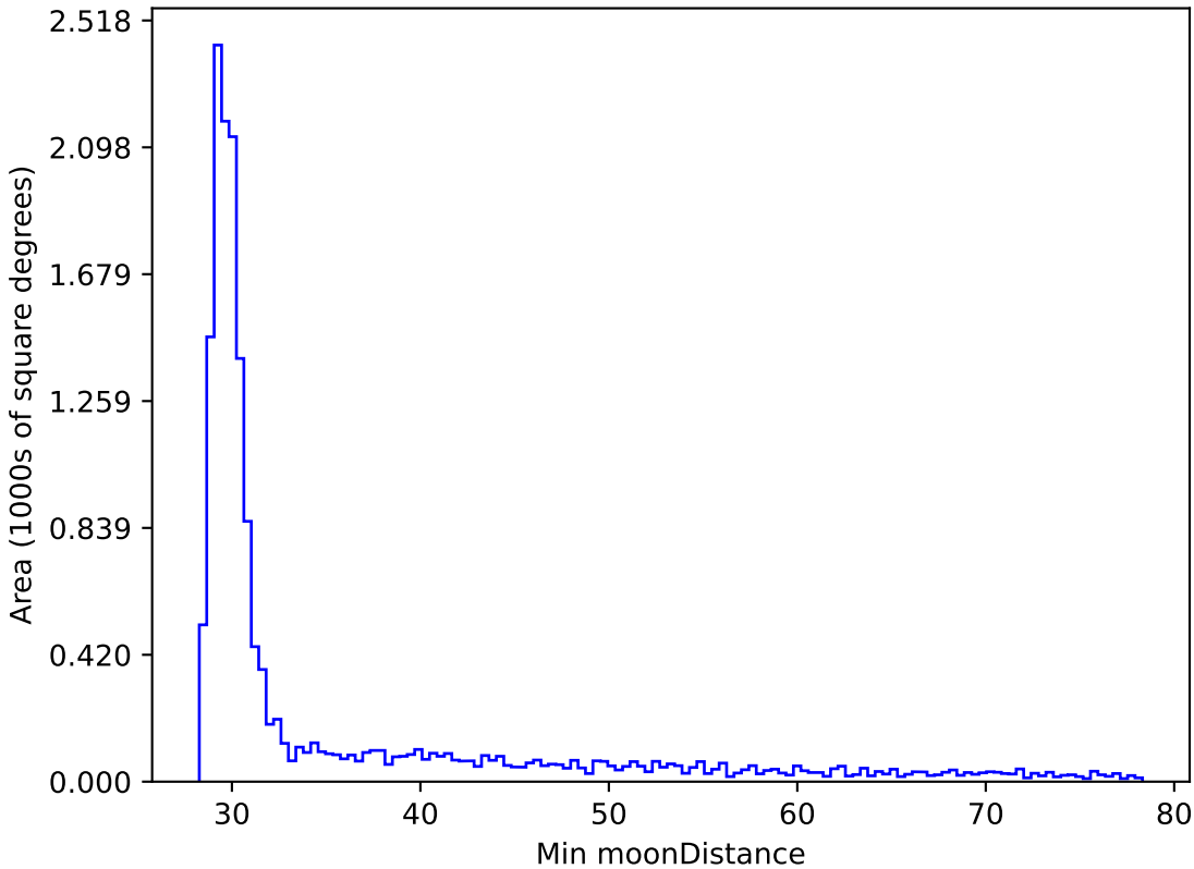
scp_reweight_v3.3_10yrs WFD z band: Min moonDistance
